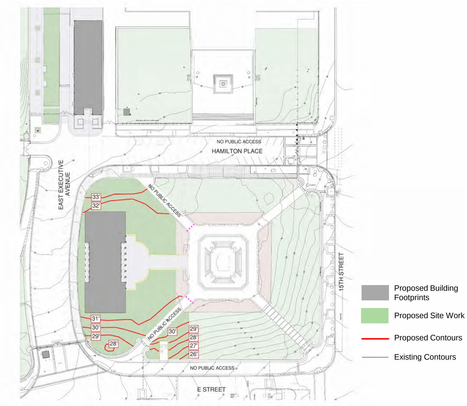
PLAN VIEW: PROPOSED SITE GRADING
