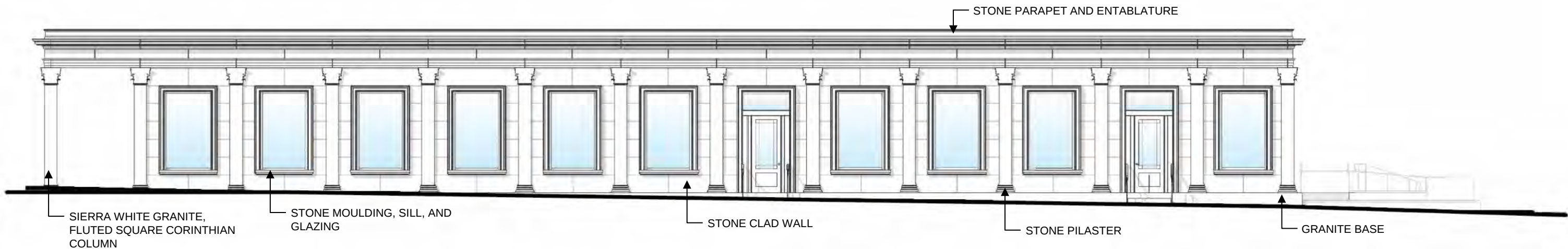
WEST ELEVATION – STAFF SCREENING / EXIT BUILDING
