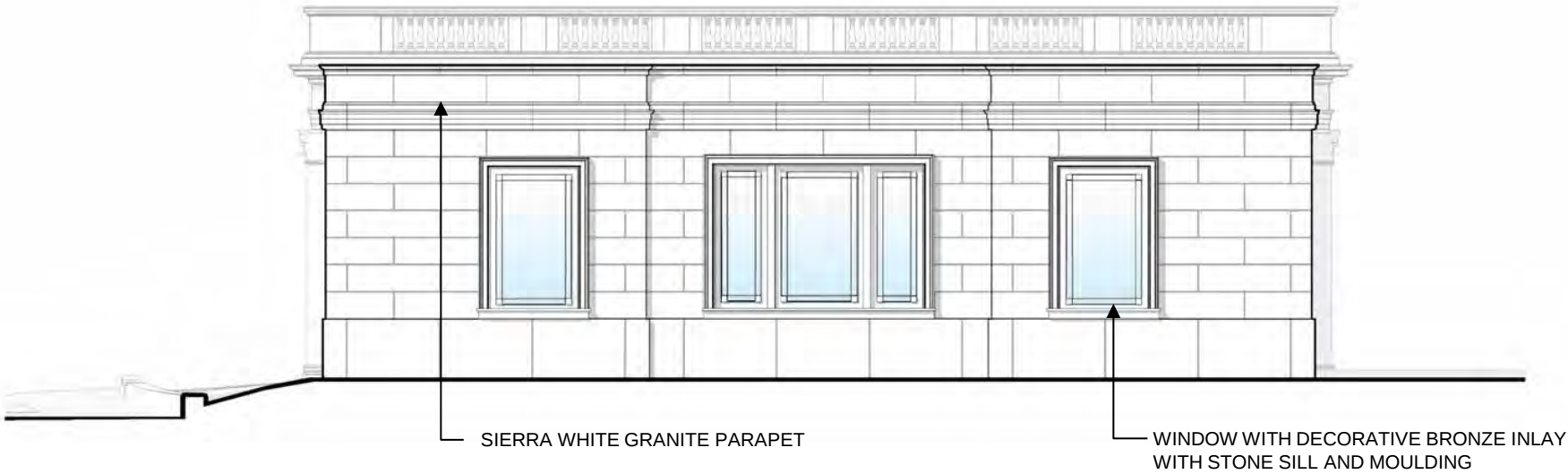
SOUTH ELEVATION - ENTRANCE PAVILION
