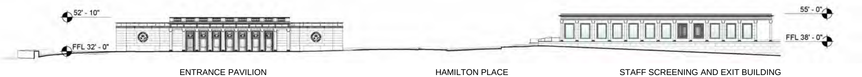
SITE ELEVATION OF EAST FACADES
