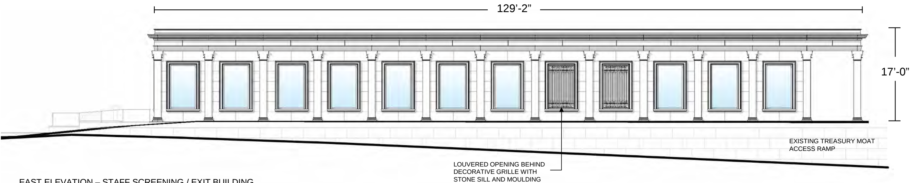
EAST ELEVATION – STAFF SCREENING / EXIT BUILDING
