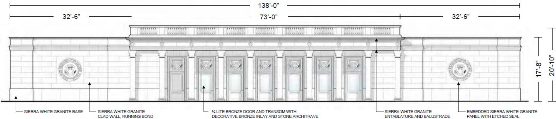
EAST ELEVATION - ENTRANCE PAVILION
