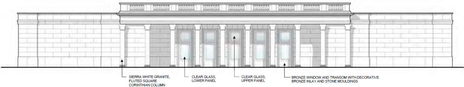
EAST ELEVATION - ENTRANCE PAVILION
