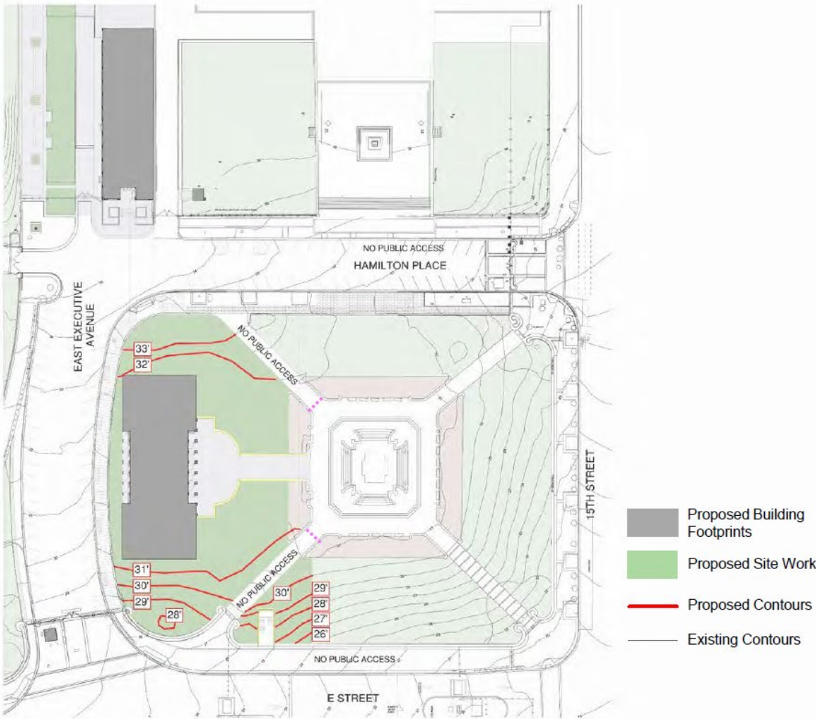
PLAN VIEW: PROPOSED SITE GRADING
