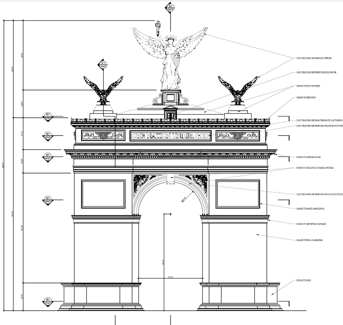
Elevations
