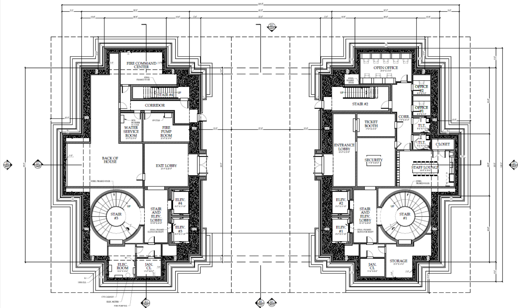
Floor plans - Base
